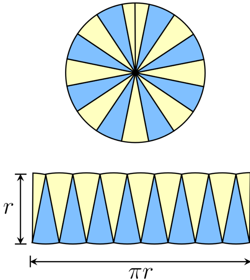
Figure 1: Area of a Circle by Sectors
